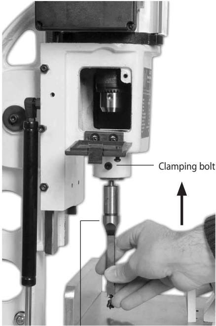
Hollow Chisel
