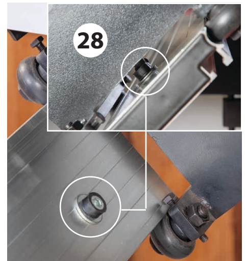
Sliding carriage stop, prevents the sliding table from coming off the carriage
