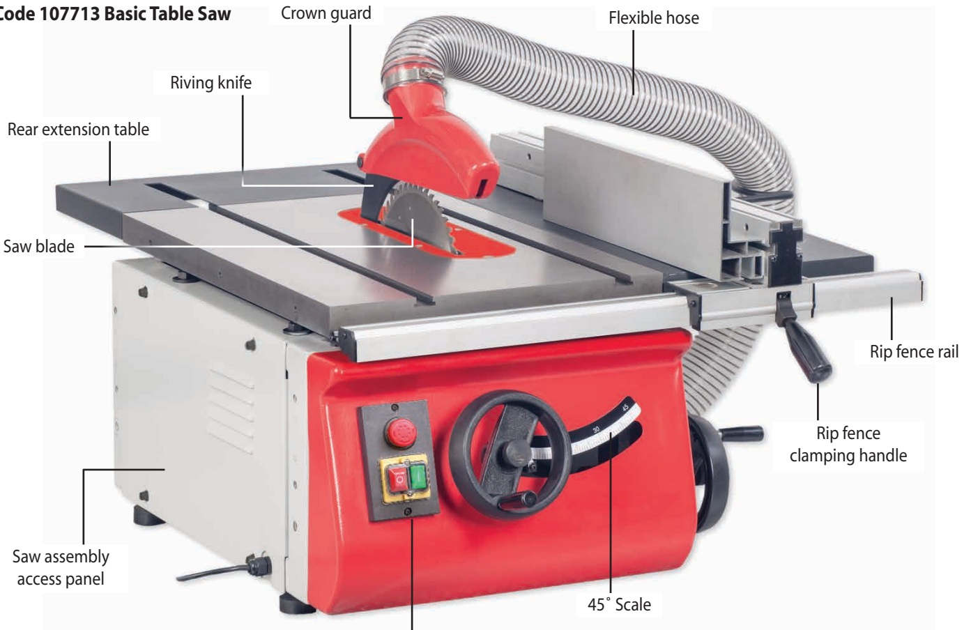
Main Table Saw
