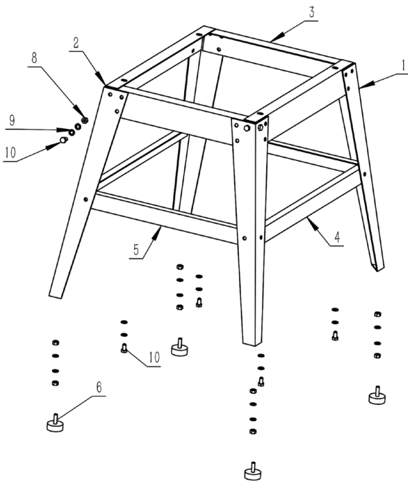
106806 AW254TS Optional Cabinet Stand Diagram D
