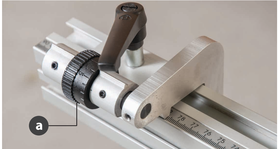
Distance stop (27) with micro adjusting wheel (a)
