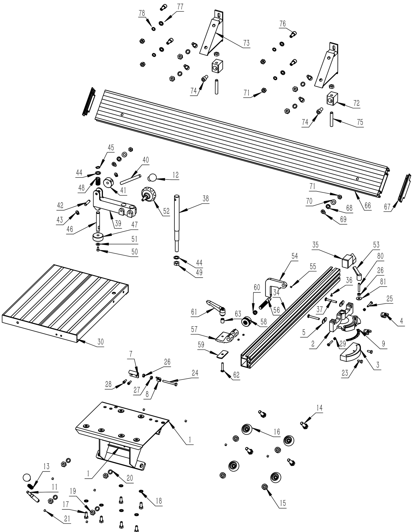
104930 AW216TS Optional Sliding Table Kit Diagram B
