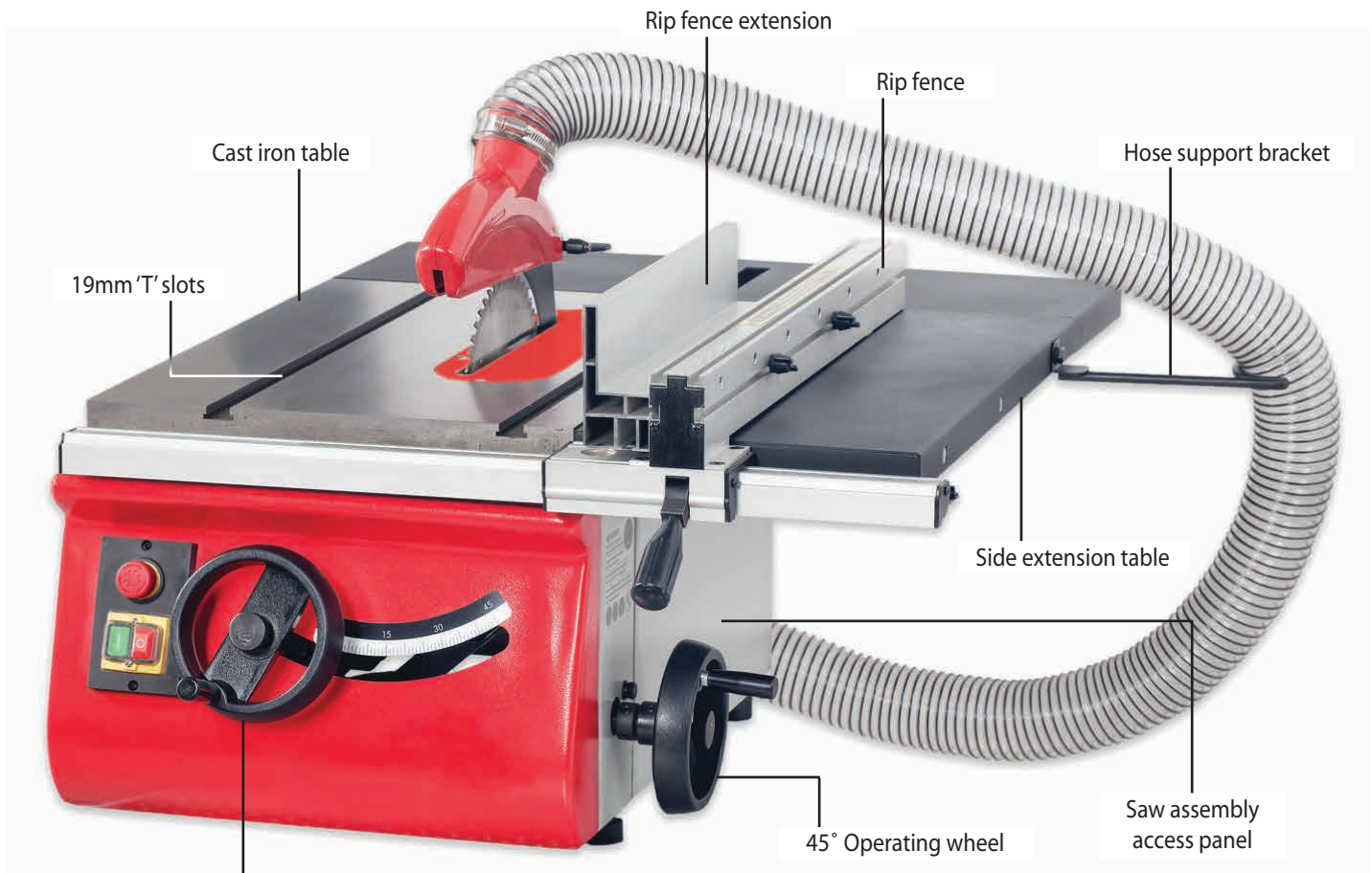
Rise & fall operating handle
