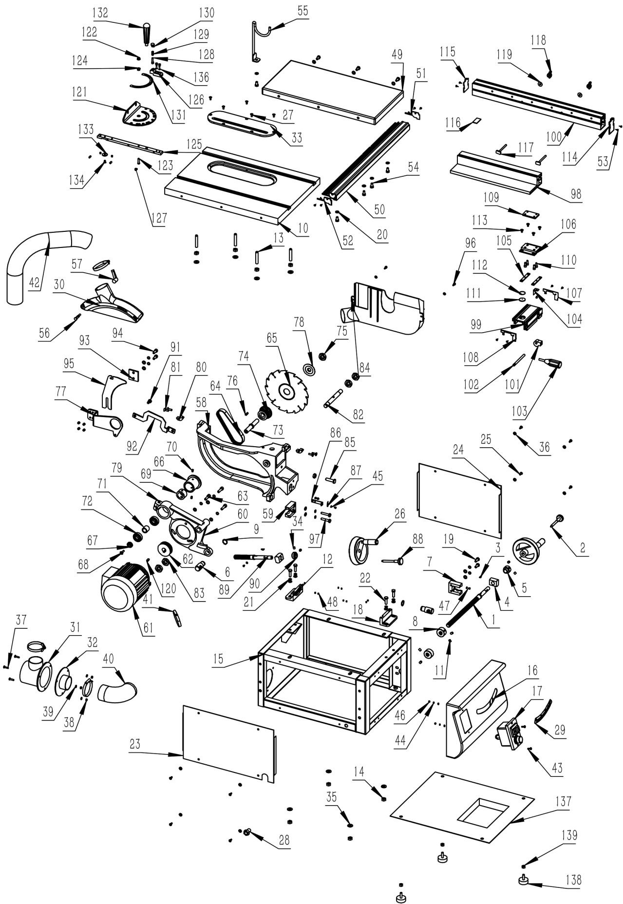
107712 AW216TS Basic Table Saw Diagram A
