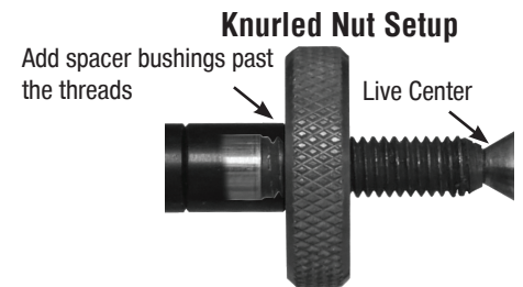
Diagram C / Bushing #PKSCERBU
