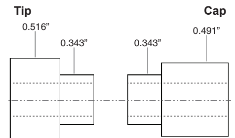
Diagram C / Bushing #PKSCERBU
