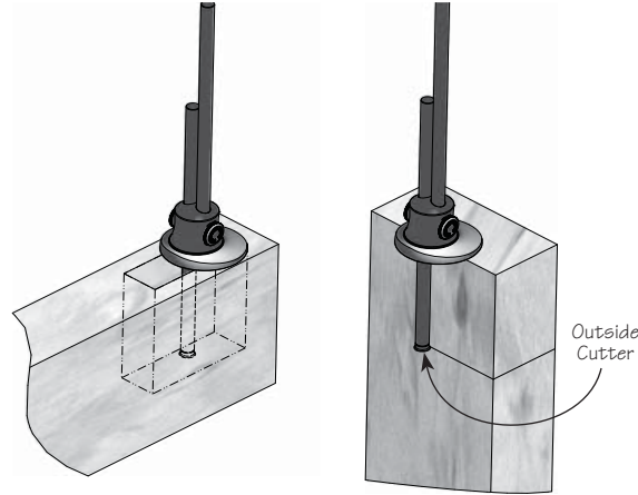
Figure 5: Transferring dimensions.
