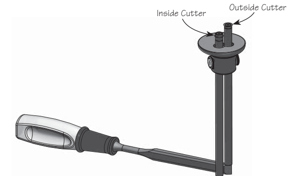
Figure 3: Setting cutters to match chisel thickness.
